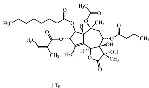
Figure 1. Structure of thapsigargin (1, Tg).
