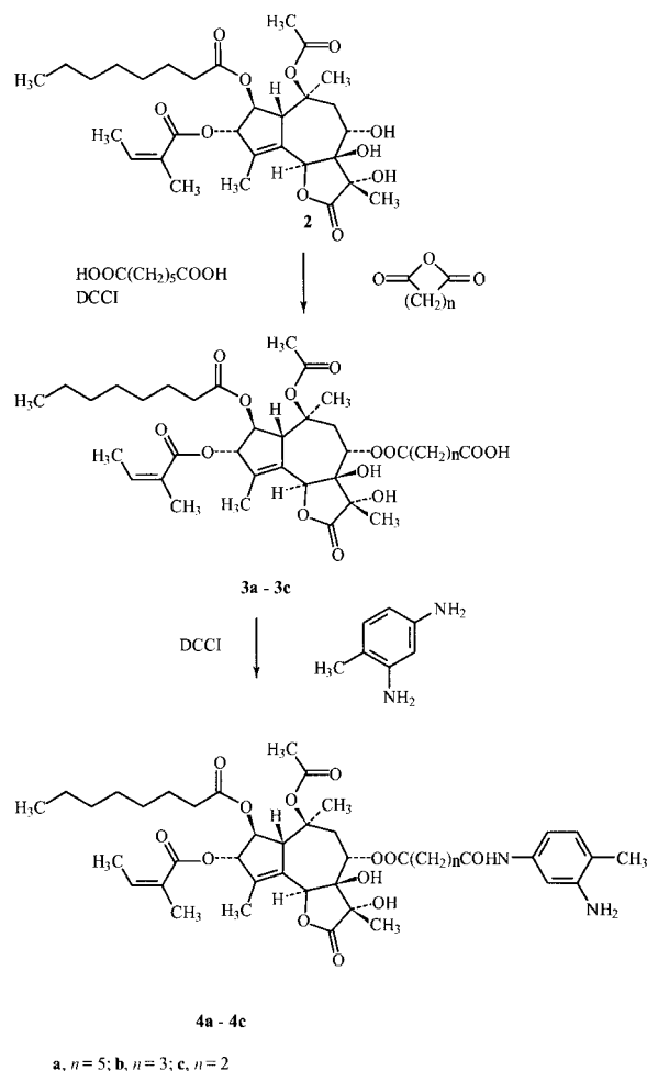
Scheme 1. Synthesis of the analogues containing a 2,4-diaminotoluene residue ( 4a–4c ).
